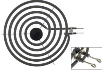
US587 (8" 2100W) Coil Surface Element Black Center Cap
