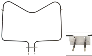
UB413 (2500W/240V) Bake Element 19"W x 15-1/2"L x 2-1/2" insert
