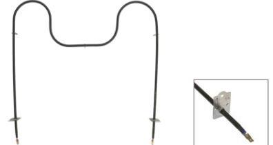
UB403 (2800W/240V) Bake Element 19"W x 19"L x 3-1/2" insert
