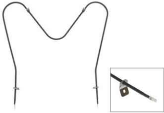
UB467 (1950/2600W/240V) Bake Element 19-1/2"W x 18-1/2"L x 3-1/2" insert
