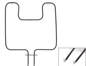
UB400 (2400W/240V) Bake Element 14-3/4"W x 14-5/8"L x 3-3/8" insert
