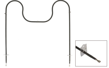
UB630 (2800W/240V) Bake Element 21-1/8"W x 15-3/8"L x 3" insert
