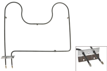
UB404 (2585W/240V) Bake Element 18-7/8"W x 15-7/8"L x 3-1/4" insert
