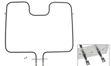
UB593 (3000W/240V) Bake Element 18"W x 13"L x 1-7/8" insert
