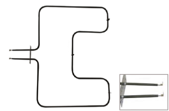
UB750 (3000W/240V) Bake Element 20"W x 15.5"L x 3-1/2" insert
