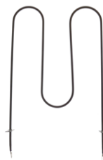
UT730 (3000W/240V) Broil Element 12"W x 15-1/4" L
