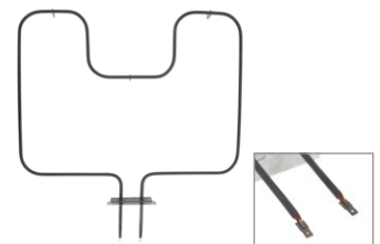
UB640 (3000W/240V) Bake Element 18-3/8"W x 16"L x 3-7/8" insert
