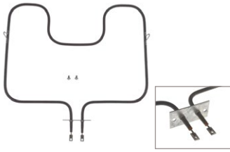
UB300 (2000W/240V) Bake Element 13"W x 11-7/64"L x 1-7/8" insert.
