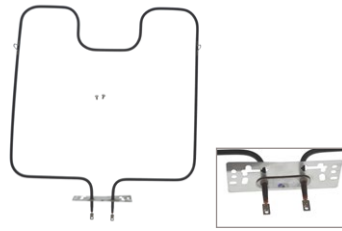
UB484 (2500W/240V) Bake Element 15-11/20"W x 15-3/8"L x 1-7/8" insert
