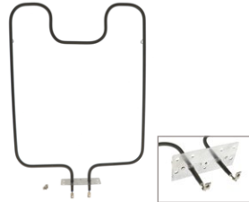
UB323 (3000W/240V) Bake Element 13"W x 16-35/64"L x 1-7/8" insert
