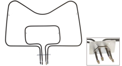
UB417 (1100/2500W/250V) Bake Element 20-1/2"W x 15-1/4"L x 2-1/4" insert
