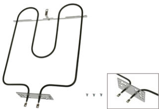
UT096 (3000W/240V) Broil Element 11"W x 16-3/64" L x 1-7/8" insert
