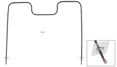
UB873 (2500W/240V) Bake Element 21-1/4"W x 16"L x 1-7/8" insert
