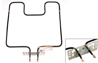
UB303 (2000W/240V) Bake Element 13"W x 14-11/20"L x 1-7/8" insert
