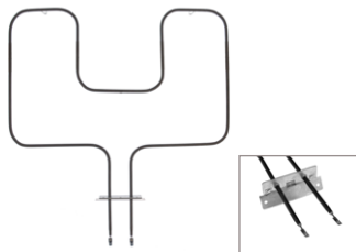
APWG02F05396 (3000W/240V) Bake Element 18-7/8"W x 15-1/4"L x 4-3/8" insert
