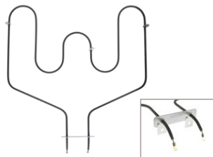
APWG02F04464 (3410W/240V) Bake Element 18"W x 16-7/8"L x 2-3/8" insert
