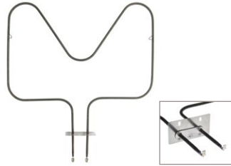
UB425 (2300W/240V) Bake Element 17"W x 19-1/2"L x 2-1/2" insert
