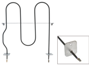
UT525 (2500W/240V) Broil Element 14-1/2"W x 16-3/4" L x 2-1/2" insert
