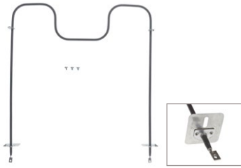
UB483 (2200W/240V) Bake Element 15-35/64"W x 16"L x 1-7/8" insert
