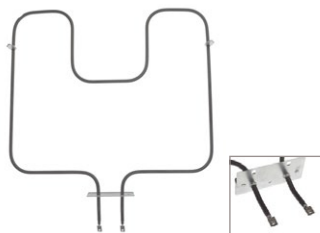
UB482 (2500W/240V) Bake Element 15-35/64"W x 14-35/64"L x 3-7/8" insert
