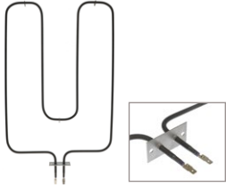
UB494 (2500W/240V) Bake Element 13"W x 17-3/4"L x 2-1/4" insert
