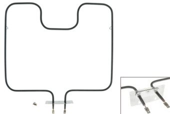
UB474 (2500W/240V) Bake Element 15-35/64"W x 14-35/64"L x 1-7/8" insert
