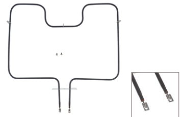
UB642 (3000W/240V) Bake Element 18-1/2"W x 14-35/64"L x 3-7/8" insert
