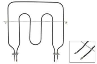
UB527 (3600W/240V) Bake Element 18"W x 12"L x 3-1/2" insert
