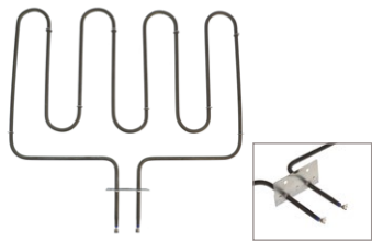
UB725 (3400W/240V) Bake Element 19-1/2"W x 15-1/2"L x 3-1/2" insert
