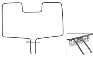
UB963 (3000W/240V) Bake Element 22-1/2"W x 14-35/64"L x 3-7/8" insert
