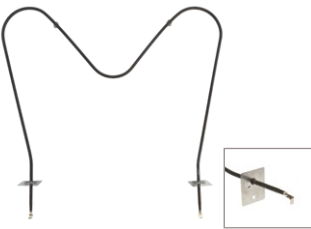
UB958 (2600W/240V) Bake Element 19-1/4"W x 15-5/8"L x 3-1/8" insert
