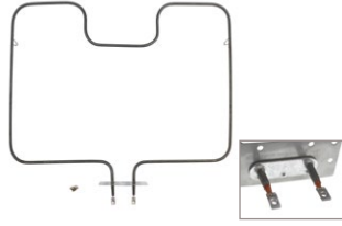
UB732 (3000W/240V) Bake Element 19-1/4"W x 15-35/64"L x 1-7/8" insert
