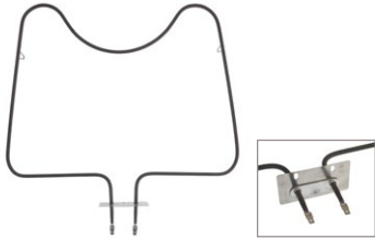
UB414 (2200W/240V) Bake Element 16-7/8"W x 14-1/2"L x 2-3/8" insert
