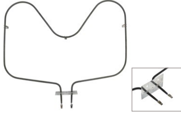
UB308 (2400W/240V) Bake Element 20-7/8"W x 15-1/2"L x 2-5/8" insert
