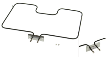
UB813 (2500W/240V) Bake Element 20-1/4"W x 14-35/64"L x 3-7/8" insert
