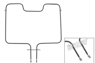
UB481 (2100W/240V) Bake Element 15-35/64"W x 14-35/64"L x 3-3/8" insert
