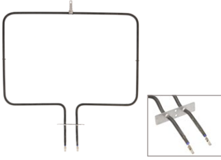
UB577 (3600W/240V) Bake Element 20-1/2"W x 16-1/2"L x 3-1/2" insert
