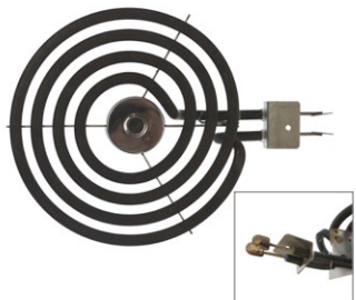
APP1T15F (6" 1500W) APP1T23F (8" 2100W) Coil Surface Element, Spade Ends Chrome Center Cap Replaces older style GE Surface Elements
