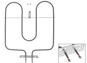
UT316 (3000W/240V) Broil Element 13"W x 15-3/64" L x 1-7/8" insert
