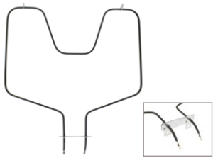
APWG02A00493 (3000W/240V) Bake Element 14"W x 16"L x 4" insert
